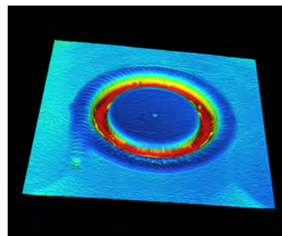
Battery sealing pin
