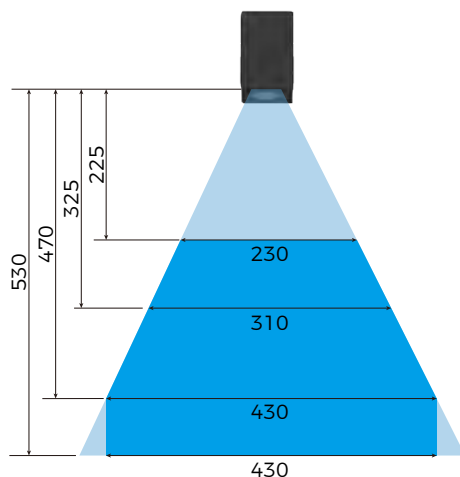
Mech-Eye LNX-8300
